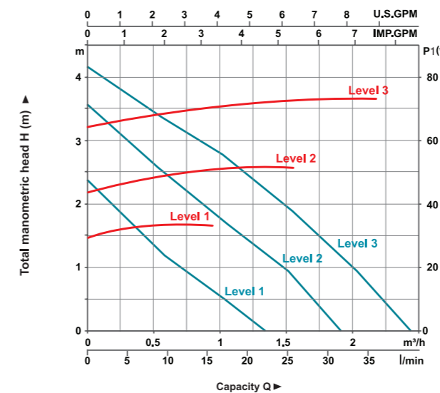
LRP15-40B/130 LRP15-40/130 — Q-H — Q-P
